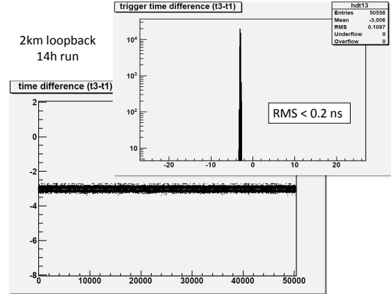
Figure 5: Time difference between PPS pulses from clock-master (WR-switch) and WR-node, T_{WRS} and T_{SPEC} (y-axis, in ns) for 2 km fiber length, as function of time (x-axis, in sec), for a 14 hr run. The histogram gives the distribution with rms < 0.2 ns.
