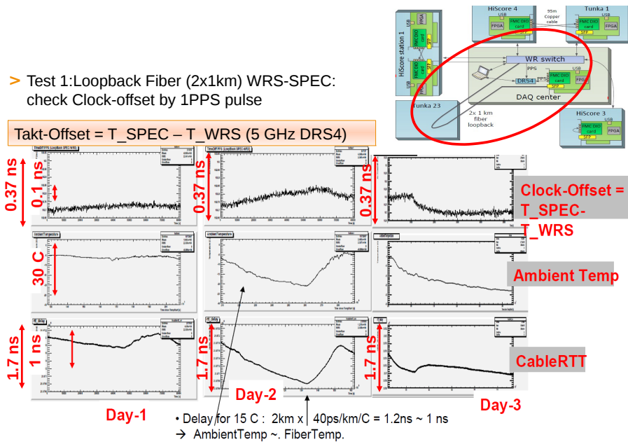
Figure 6: In-situ measurement of the sub-nsec WR-clock-stability by tracing the PPS-signal time difference between clock-master (WR-switch: T_{WRS} ) and a WR-node (SPEC card: T_{SPEC} ) (upper panel), averaged over 1000 sec. Test interval shown is three consecutive days, environmental fiber temperature changes were up to 30^{\circ}\text{C} (middle panel), which result in fiber-propagation delays (Cable-RTT) of up to 1.5 ns (lower panel).
