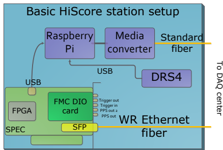
Figure 2: The basic White Rabbit setup, as contained in each HiSCORE prototype station: WR-node (SPEC card) with WR-fiber, Raspberry Pi and DRS4.
